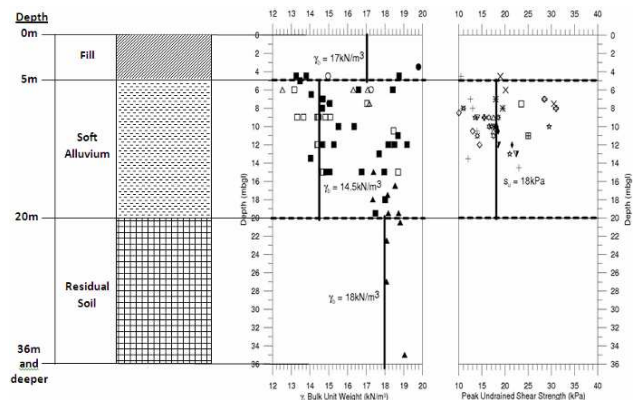
Figure 1 Established Geotechnical Model for Analysis
