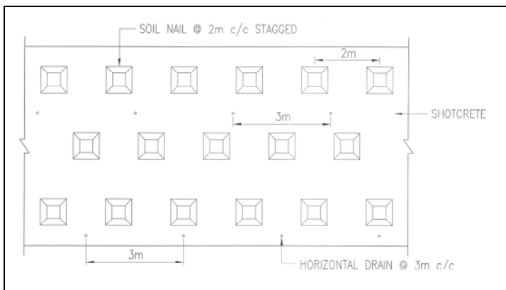
Figure 6 Shotcrete/Gunite Facings
