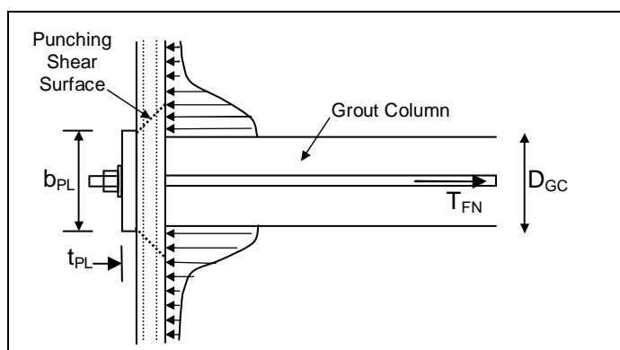
Figure 4 Typical Punching Shear of Bearing Plate Connection
