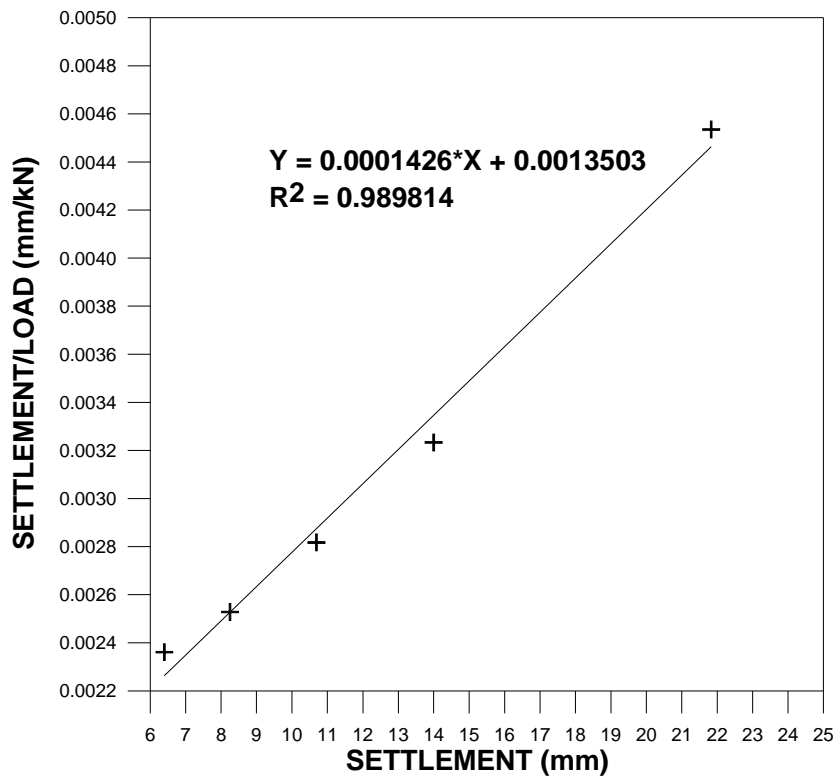
Figure 13. Chin's plot for \phi 500\text{mm} spun pile (Site D).
