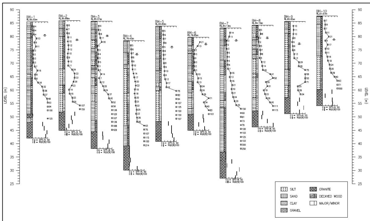
Figure 7. Borehole profiles at Site C.
