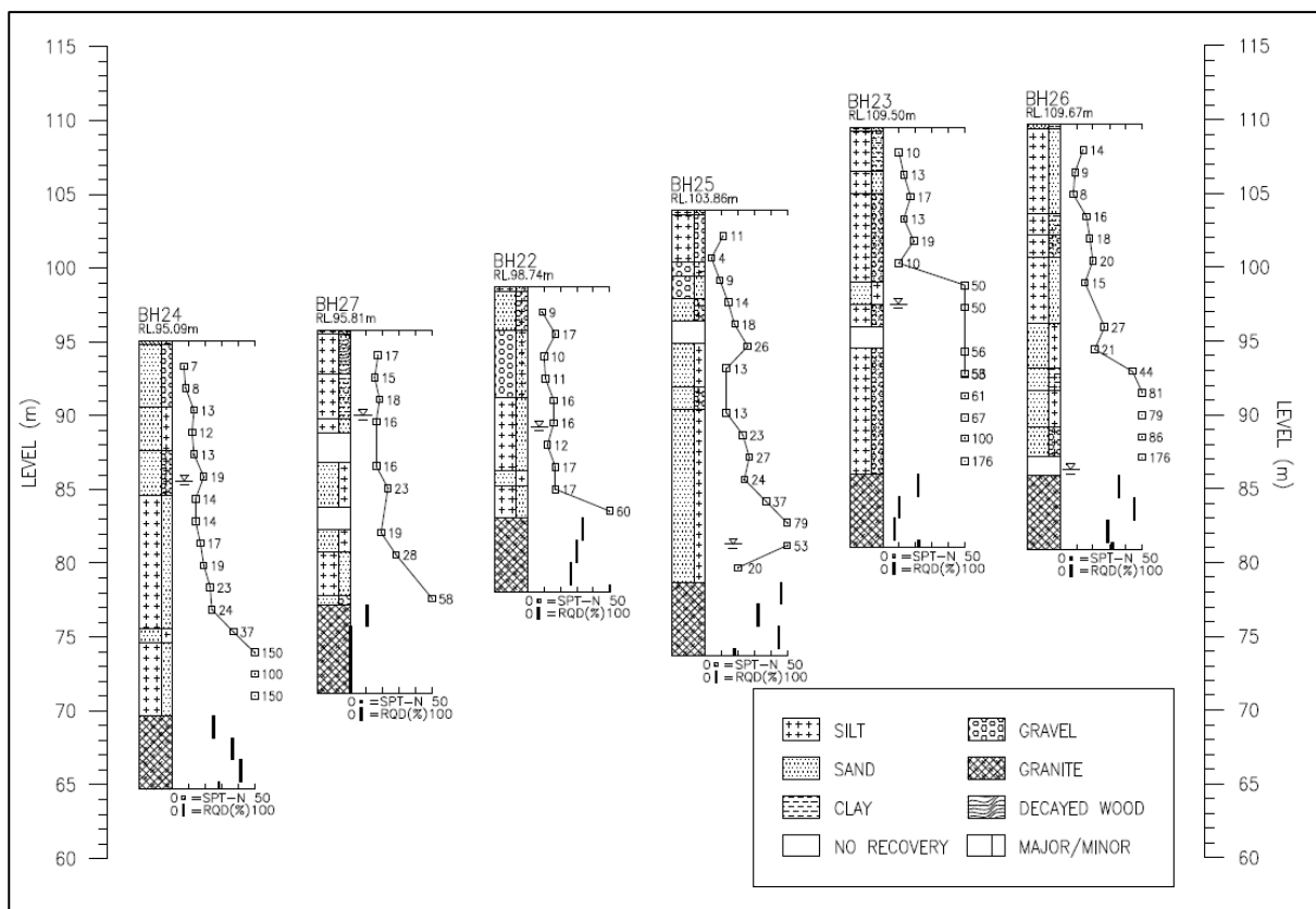
Figure 6. Borehole profiles at Site B.
