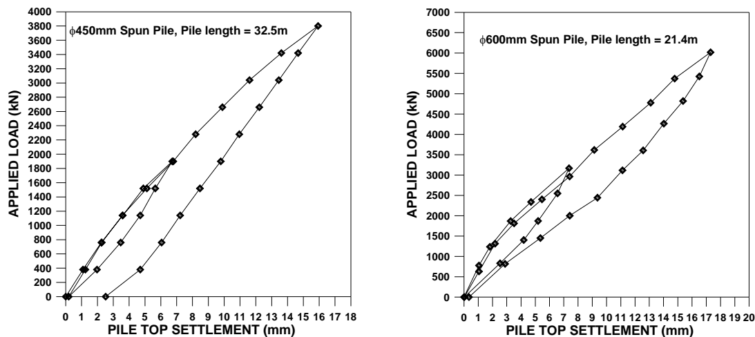
Figure 11. Load-settlement results of pile load test at Site C.
