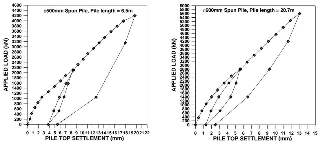
Figure 10. Load-settlement results of pile load test at Site B.
