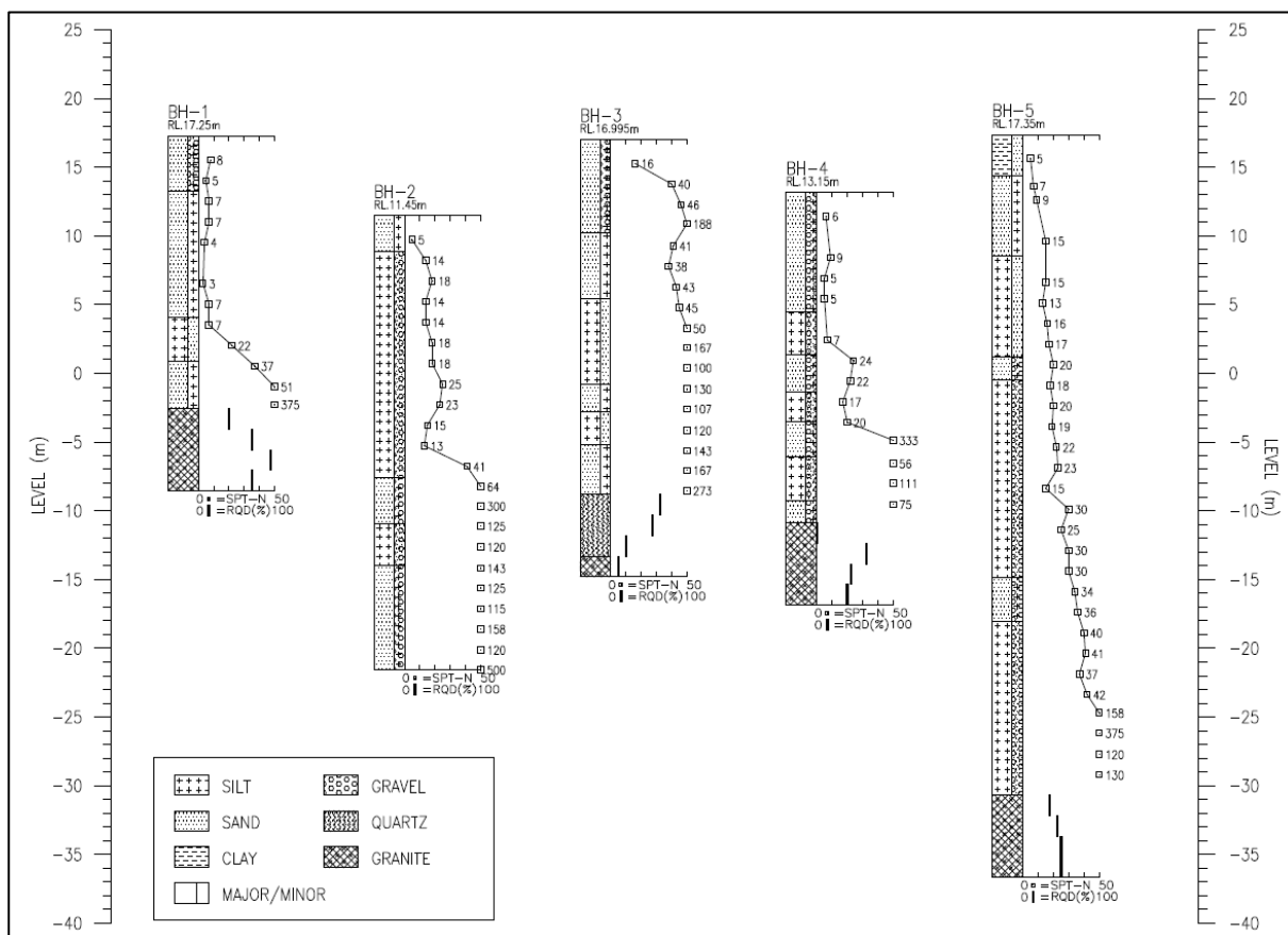
Figure 8. Borehole profiles at Site D.
