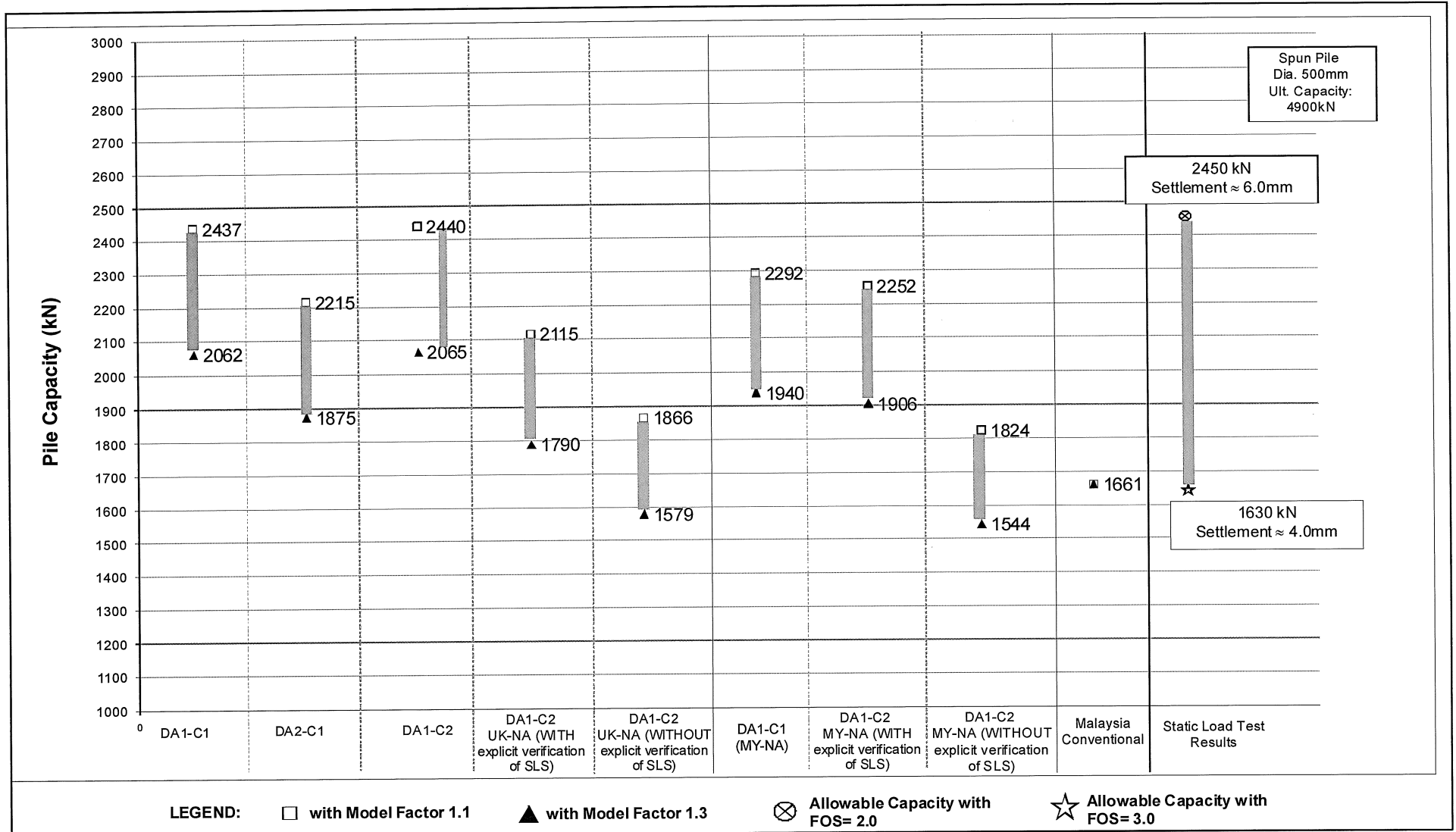
Figure 14. Allowable pile capacity of Jack-in Pile calculated using various methodologies compared with the Malaysian conventional design method and static pile load test results ( \phi 500\text{mm} Spun Pile – Site D).
