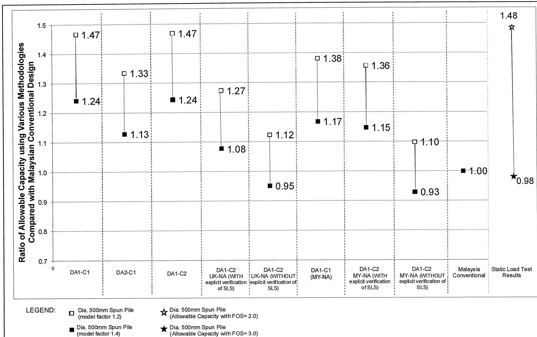
Figure 15. Ratio of Jack-in Pile allowable capacity calculated using various methodologies compared with the Malaysian conventional design method and static pile load test results.
