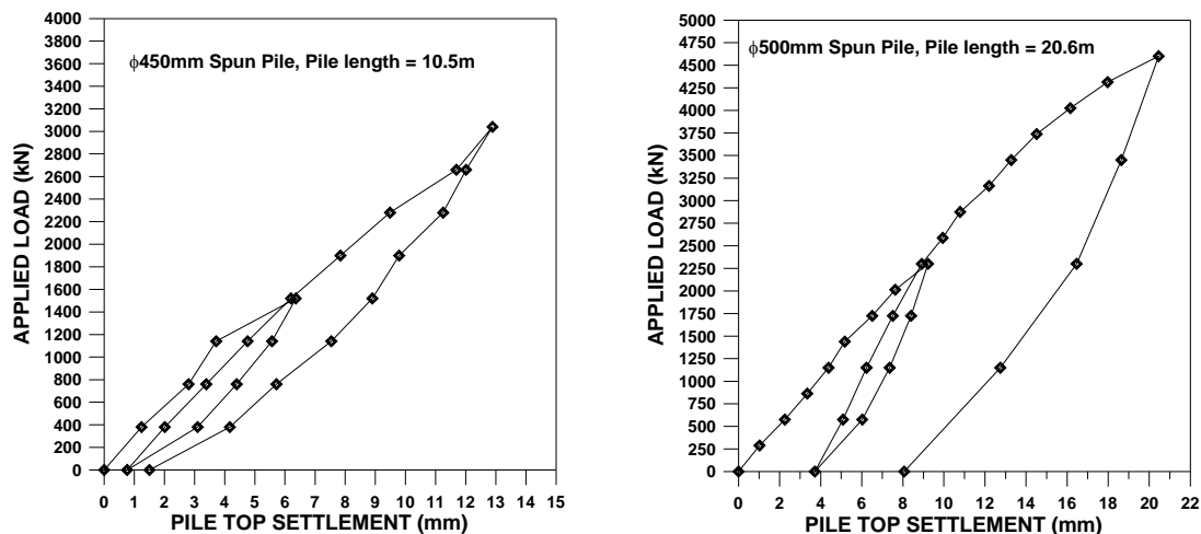
Figure 9. Load-settlement results of pile load test at Site A.
