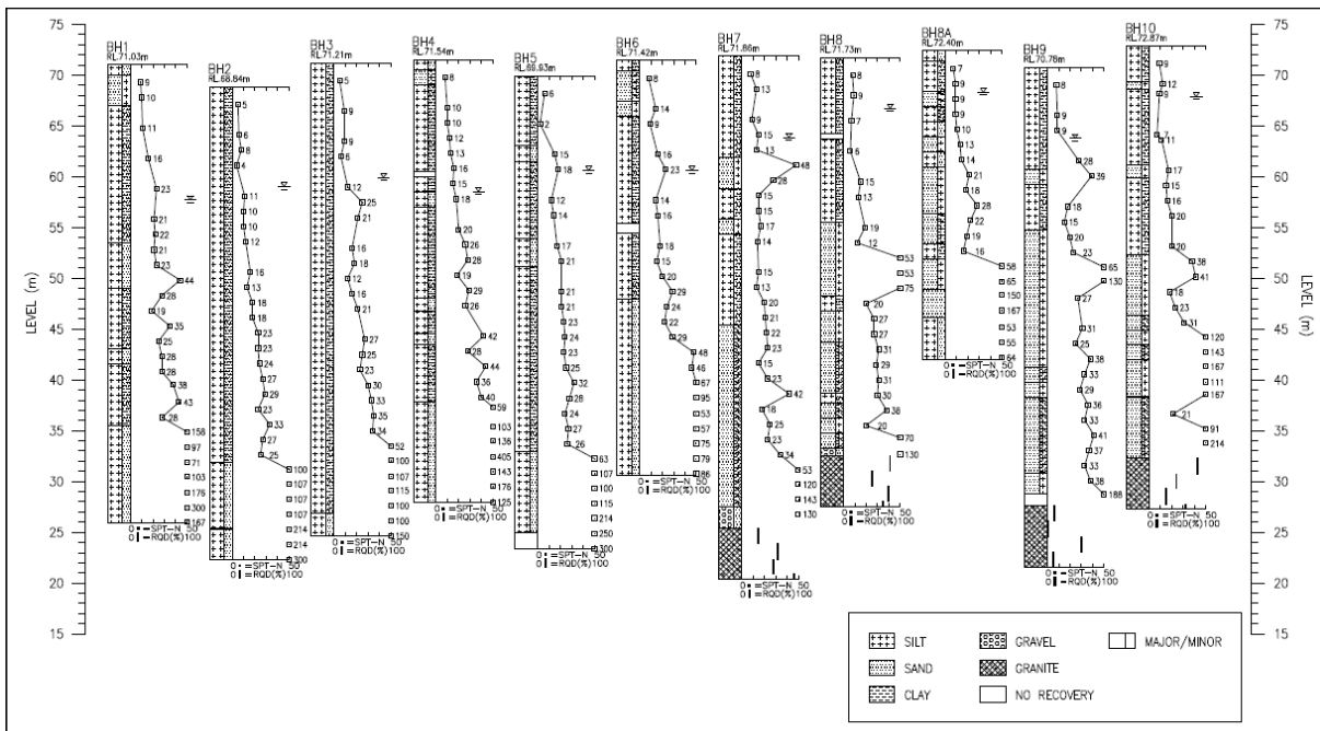
Figure 5. Borehole profiles at Site A.
