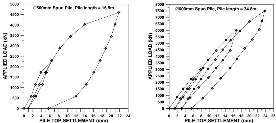
Figure 12. Load-settlement results of pile load test at Site D.
