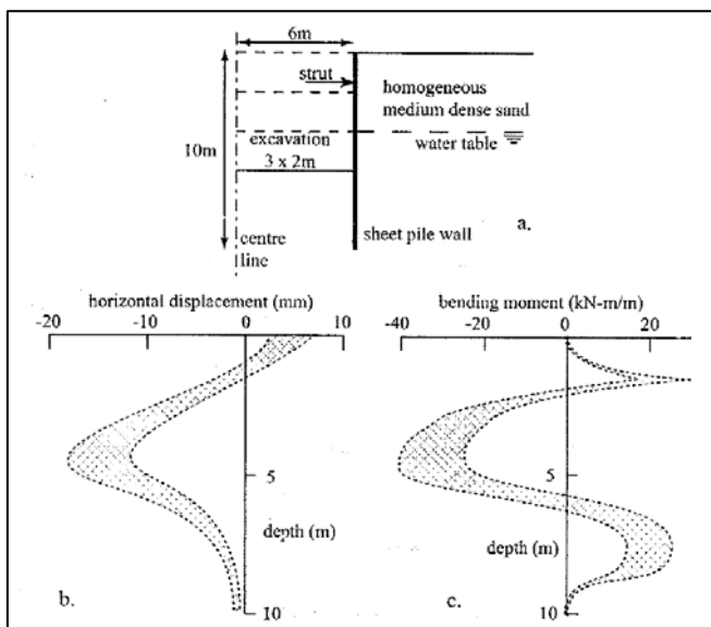
Fig. 1 Benchmark comparisons of results of numerical analysis of strutted sheet pile wall retaining dense sand using PLAXIS: (a) outline of problem analysed; (b) approximate range of predictions of horizontal displacement of walls; (c) approximate range of predictions of bending moment in walls (Wood, 2004).
