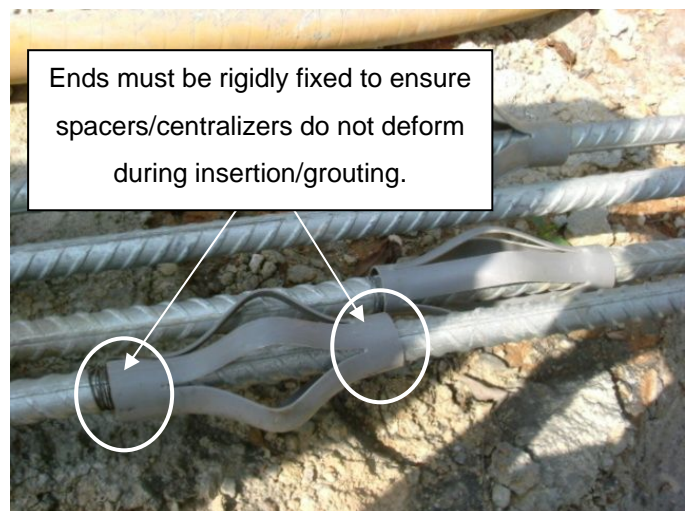
Fig. 7 Typical spacers/centralizers for soil nails.
