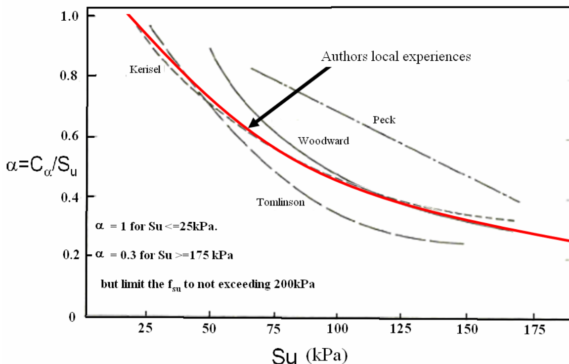
Figure 1 Adhesion factors for driven piles in clay (modified from McClelland, 1974)
