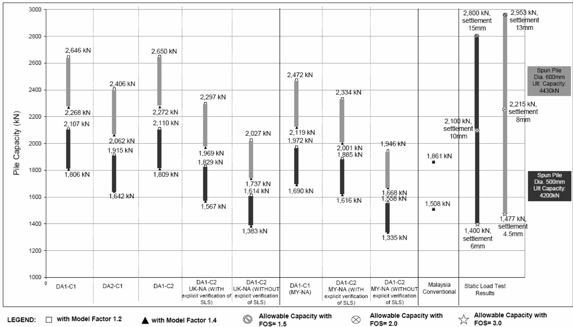
Figure 3 Allowable pile capacity of Driven Piles for various methodologies compared with Malaysian conventional design method and static pile load test results (500mm and 600mm size piles)
