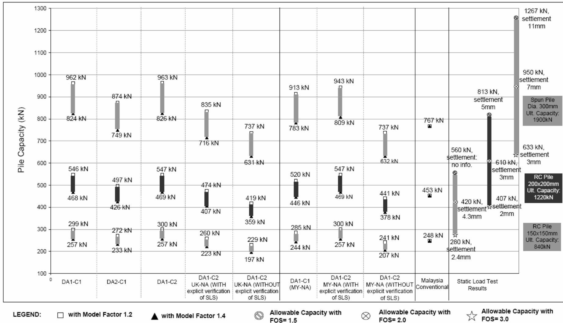
Figure 2 Allowable pile capacity of Driven Piles for various methodologies compared with Malaysian conventional design methods and static pile load test results (150mm to 300mm size piles)
