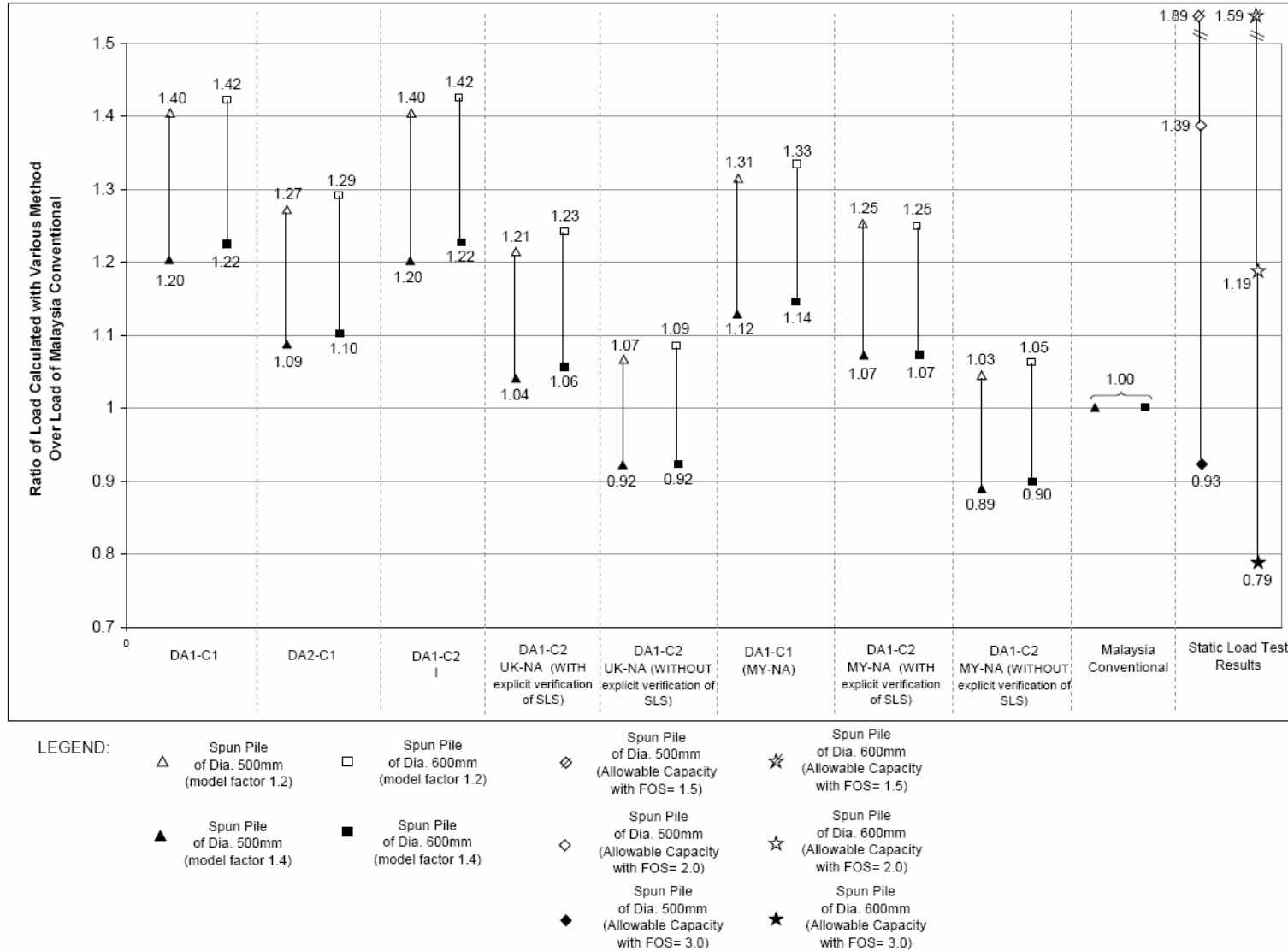
Figure 5 Ratio of Driven Pile allowable capacity for various methodologies over allowable capacity calculated via Malaysian conventional design (500mm and 600mm size piles)
