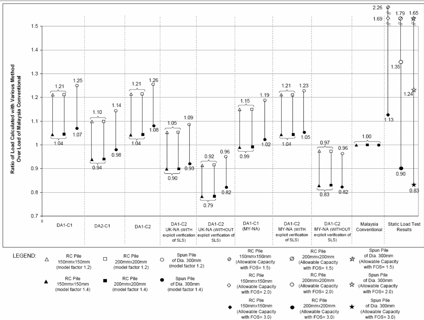
Figure 4 Ratio of Driven Pile allowable capacity for various methodologies over allowable capacity calculated via Malaysian conventional design (150mm to 300mm size piles)
