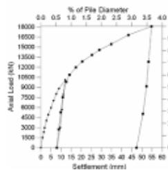
Fig. 5 Load Displacement for Test Pile A
