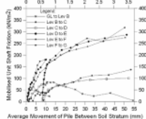
Fig. 6 Mobilised Unit Shaft Frictions for Test Pile A
