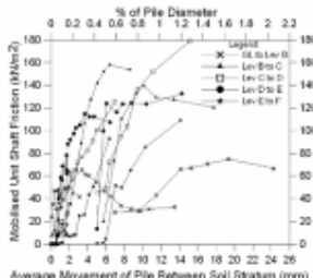
Fig. 10 Mobilised Unit Shaft Frictions for Test Pile B
